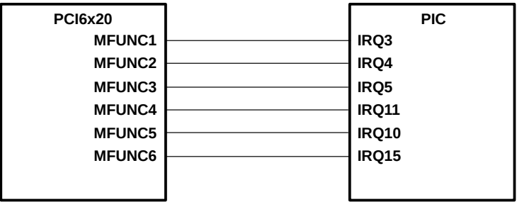
Figure 3–11. IRQ Implementation
